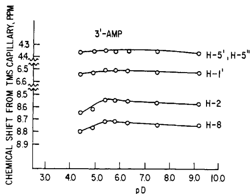
Figure 7. Chemical shift vs. pD for protons of 3'-AMP (0.09 M, 30°).
