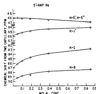
Figure 1. Chemical shift vs. molal concentration for 5'-AMP (Na) protons; 30°, D 2 O, pD 5.9.
