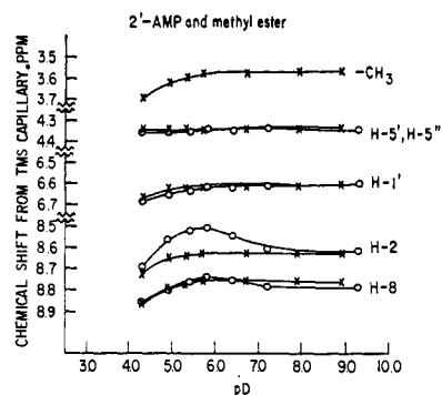
Figure 8. Chemical shift vs. pD for protons of 2'-AMP ( -\circ- , 0.09 M, 30°) and adenosine 2'-methyl phosphate ( -\times- , 0.09 M, 25°).
