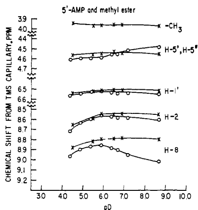
Figure 6. Chemical shift vs. pD for protons of 5'-AMP ( -\circ- , 35°, 0.08 M) and 5'-AMP monomethyl ester ( -\times- , 30°, 0.08 M).
